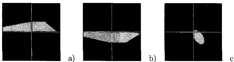
Fig. 3: a, b) The graph of skin colour cluster of the first method for the 2D skin colour determination shows: a) function C_r(Y) (first line in Eq. (2)), b) function C_b(Y) (second line in Eq. (2)). c) The skin cluster of the second method for the 2D skin colour determination: x axis of coordinate system corresponds to component C_r and y axis corresponds to component C_b (see Eq. (3)).
