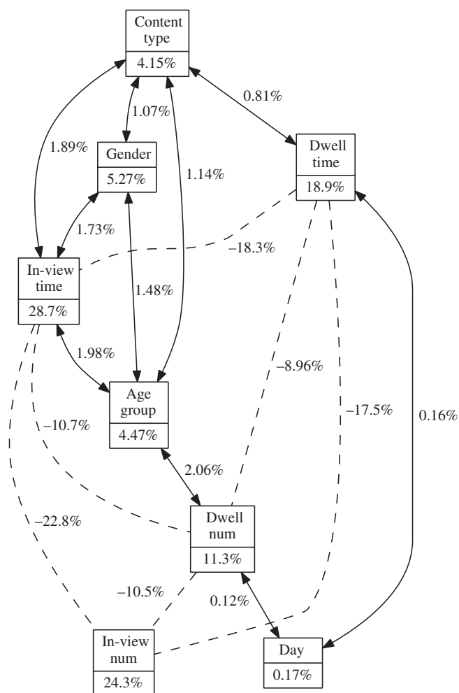
Figure 8. Interaction graph of metrics data collected in the field study.
